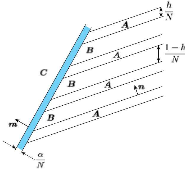
Figure 8.1: An interface separating austenite from twinned martensite. The martensitic variants are characterized by the deformation gradient tensors A, B and have volume fractions h and 1-h . The thickness of the shaded diffuse interface tends to zero as the fineness of the twin bands increases, i.e., N \rightarrow \infty .
