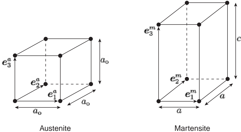
Figure 2.2: Simple cubic lattice (austenite) with lattice parameters a_0 \times a_0 \times a_0 and lattice vectors \{\mathbf{e}_1^a, \mathbf{e}_2^a, \mathbf{e}_3^a\} ; and simple tetragonal lattice (martensite) with lattice parameters a \times a \times c and lattice vectors \{\mathbf{e}_1^m, \mathbf{e}_2^m, \mathbf{e}_3^m\} .
