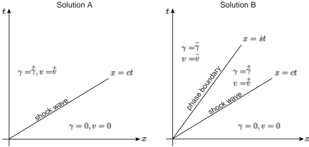
Figure 6.2: Solution forms with and without phase transition.
